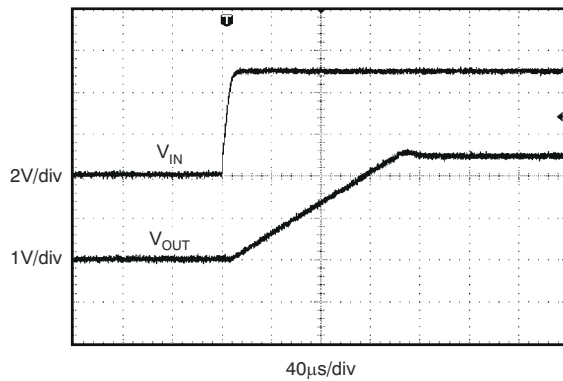
Figure 7-15. Start-Up
