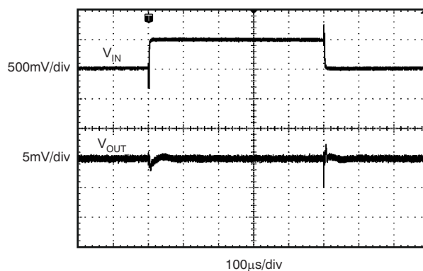
Figure 7-22. Line Transient
